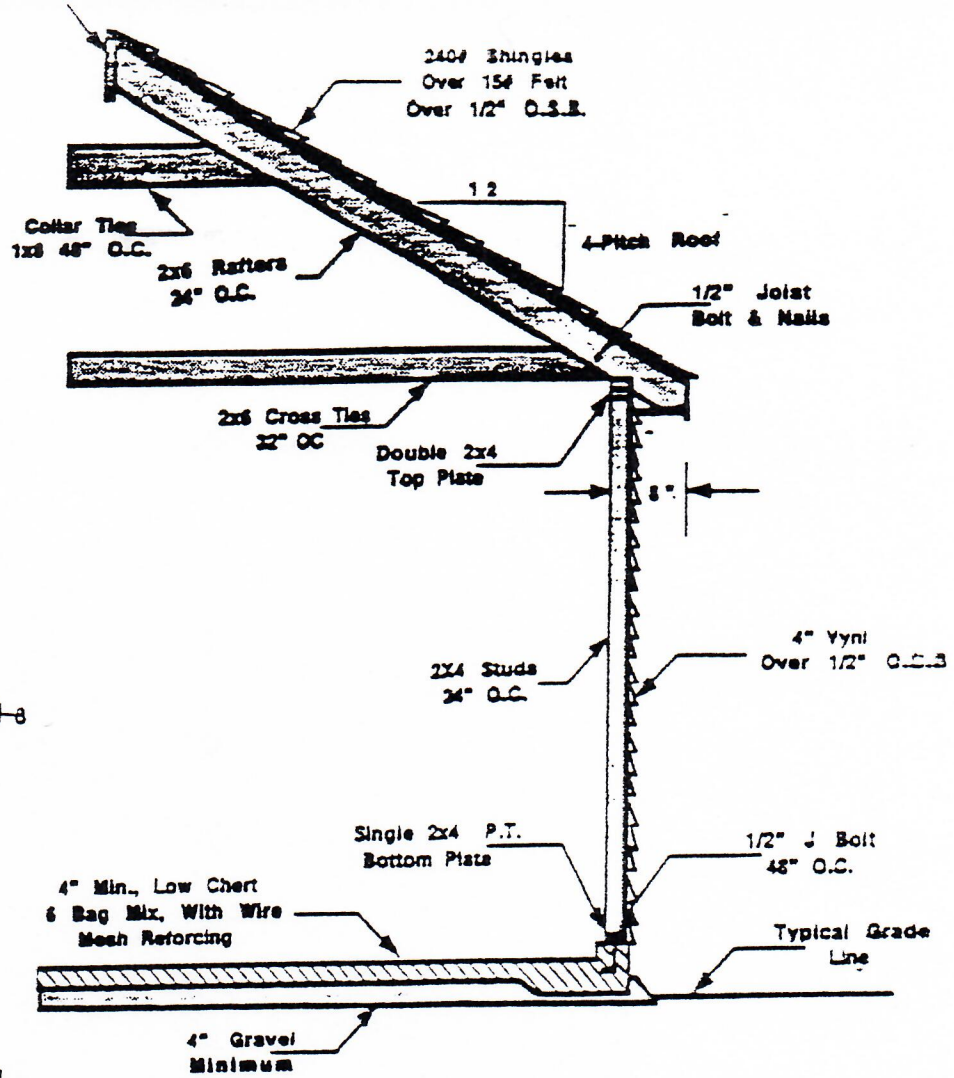
Cross Section For Gable Frame Garage
